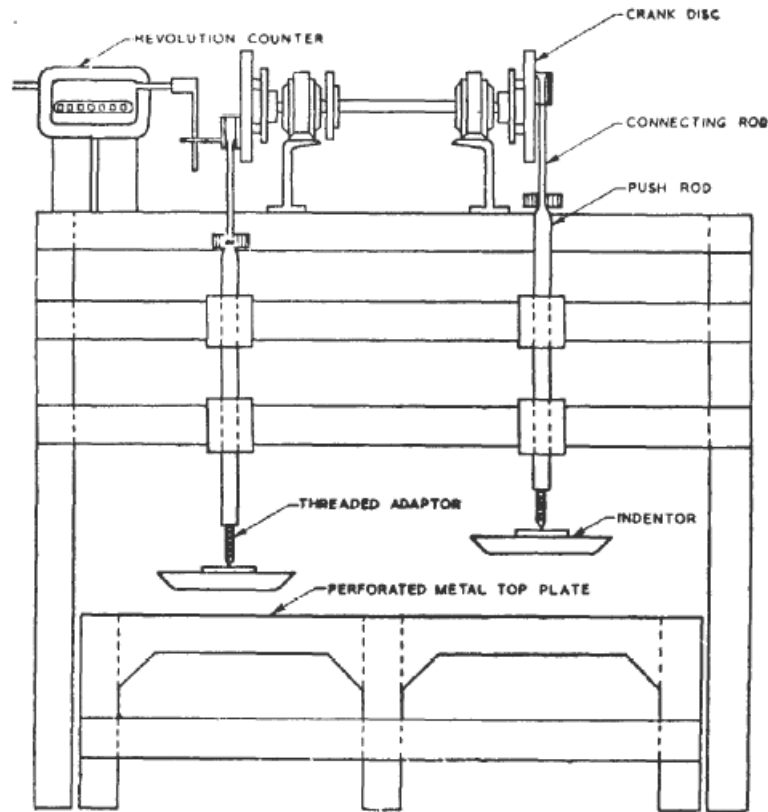
FIG. 1 APPARATUS FOR FLEXING TEST
