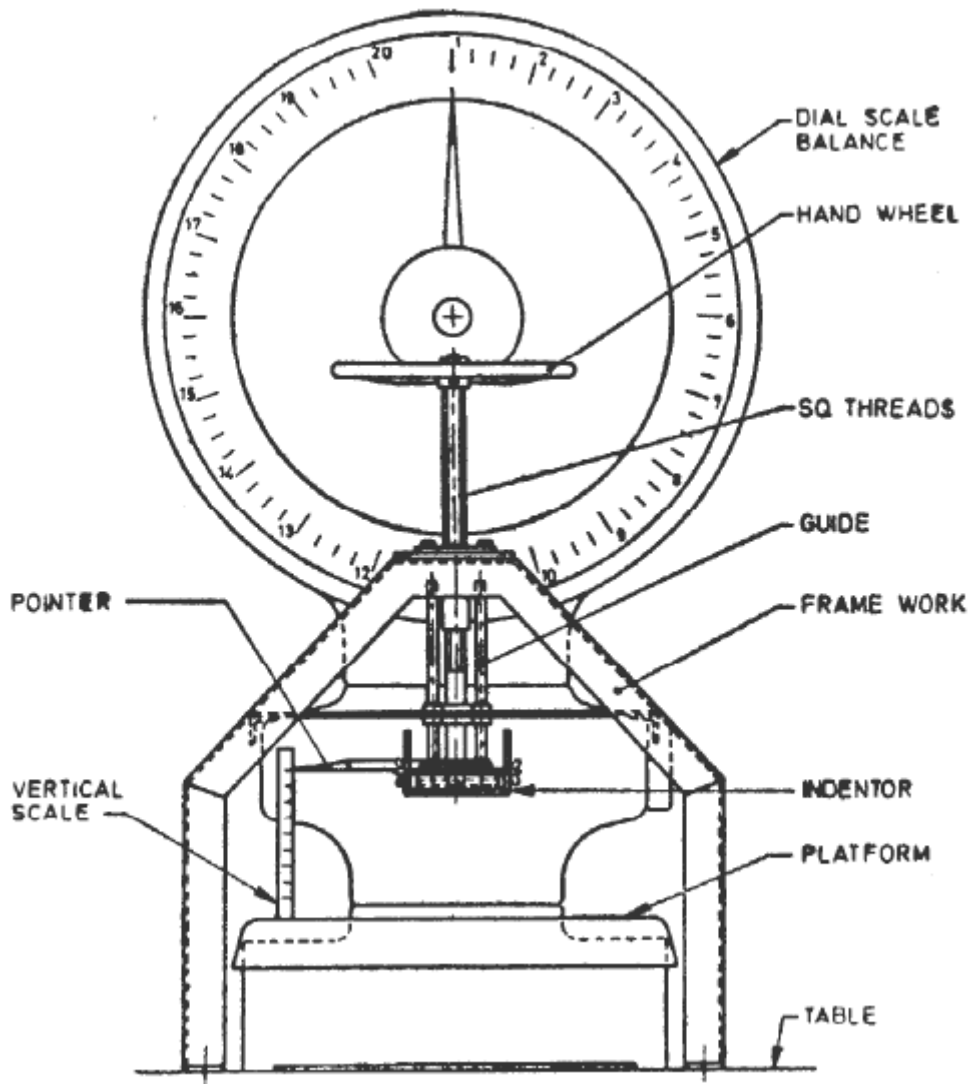
FIG. 1 APPARATUS FOR INDENTATION TEST
